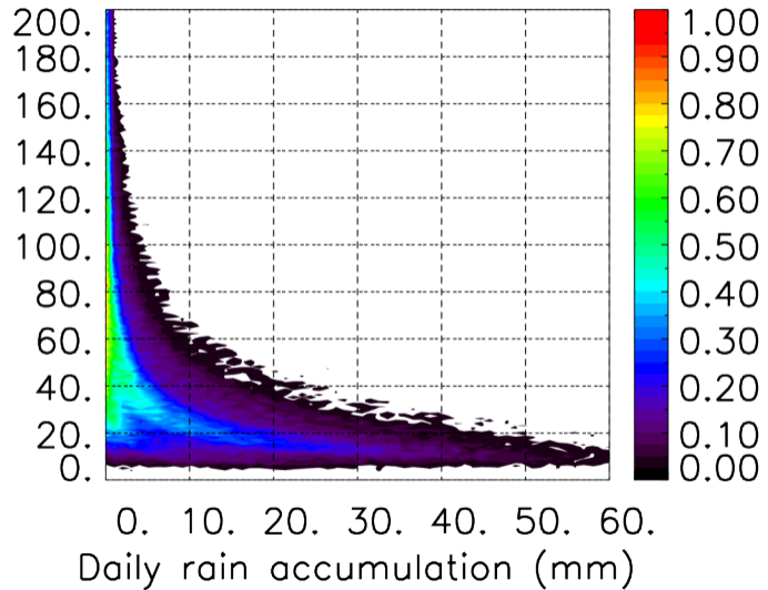
MER : 12 2020 00H
