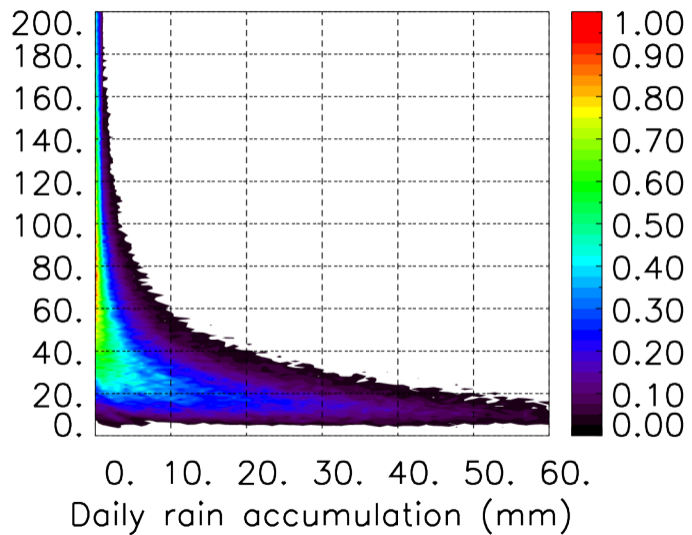
MER : 10 2020 00H
