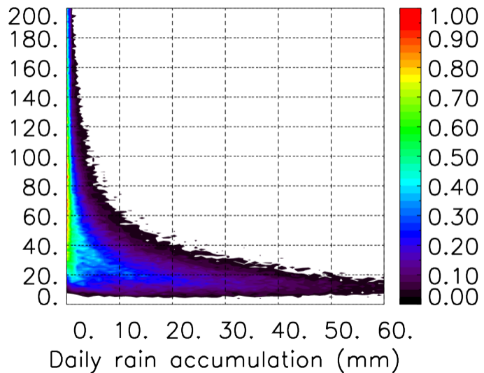
MER : 06 2020 00H
