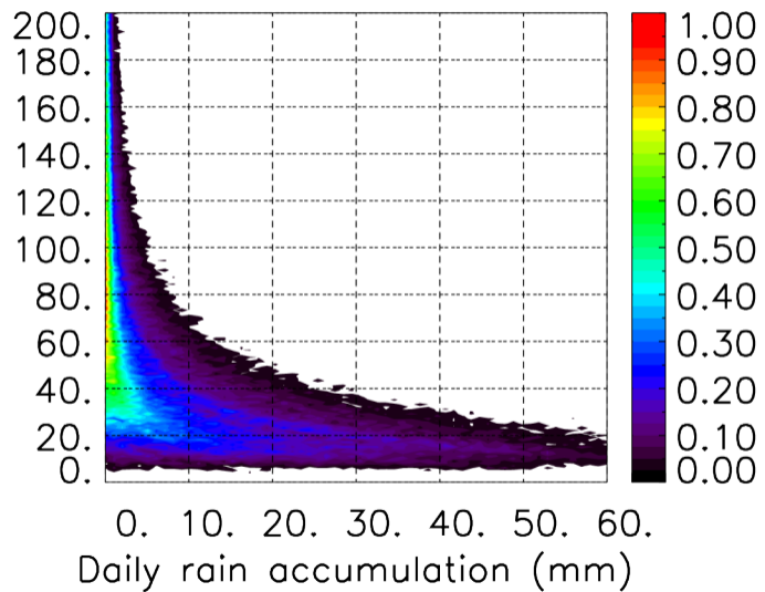
MER : 05 2020 00H
