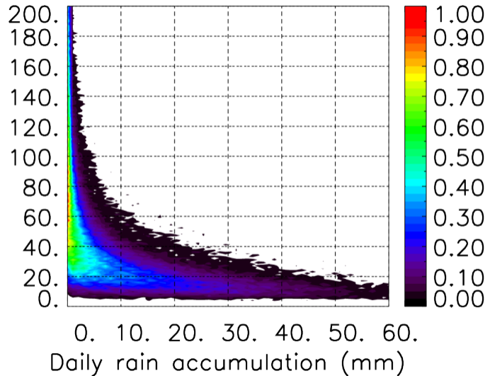
MER : 11 2020 00H
