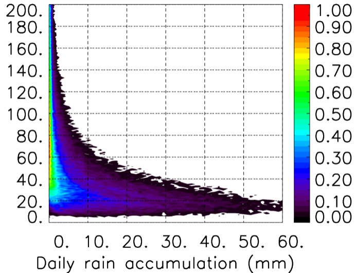
MER : 12 2015 00H
