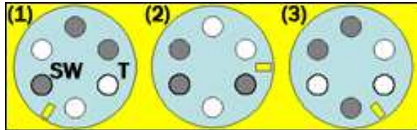
Figure 2 : ScaRaB different modes. In grey, the filters. In white no filter inside the channel. SW is for channel 2, T is for channel 3.
